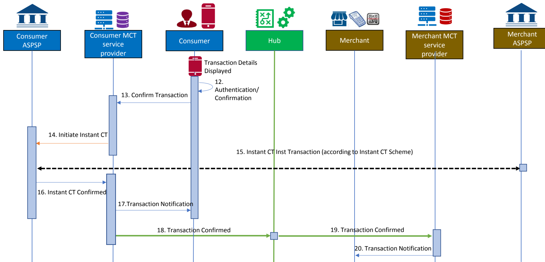
Figure 3 — Process flow – Merchant-presented QR-code with token
